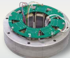
Xcelflux™ Magnetic Bearing
